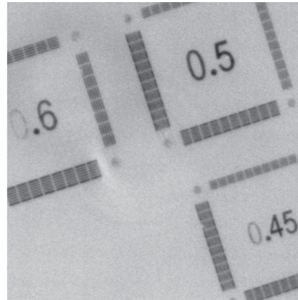
Nanofocus Resolution Miniscule focal spots in the sub-micrometer range allow to resolve even finest details and obtain clear images.
